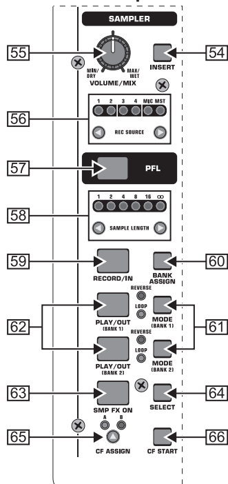
Fig. 2.6: Sampler section
