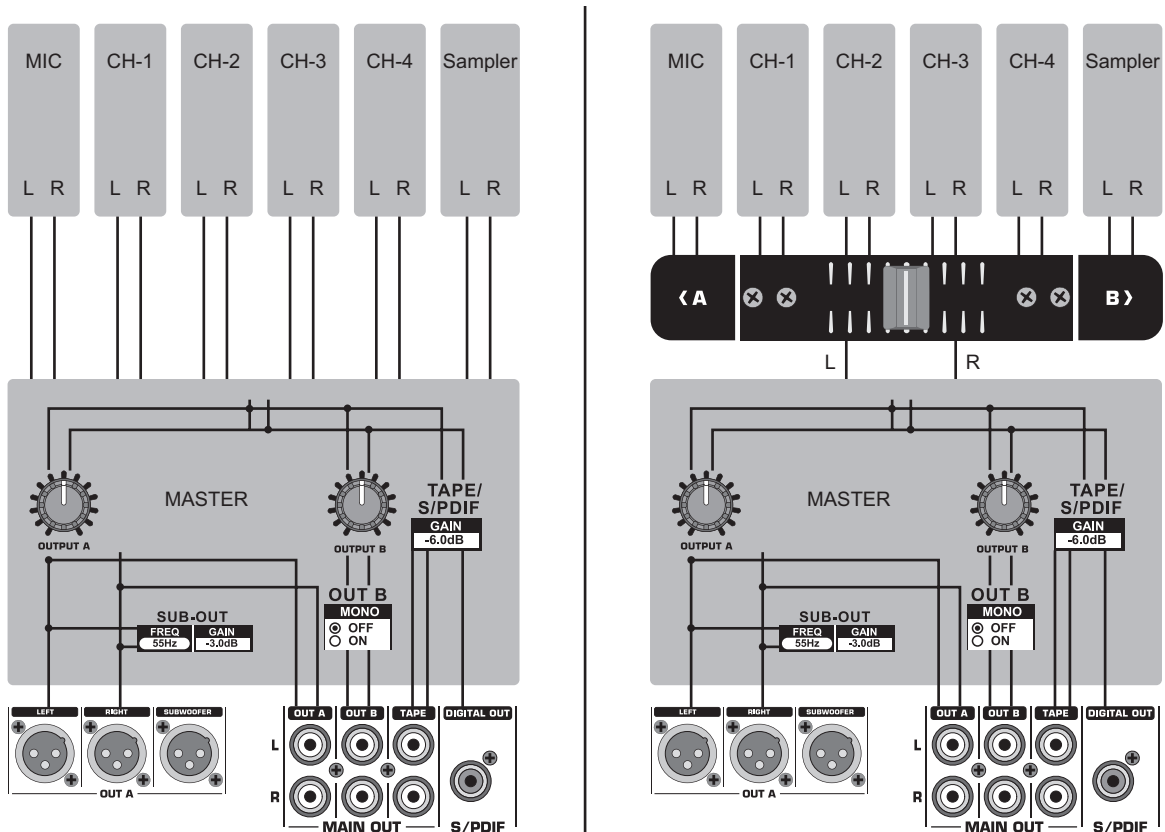
Fig. 10.2: Mixer routings
