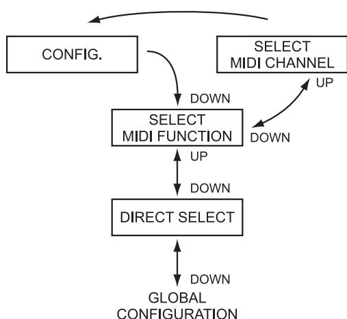
Fig. 2.3: GLOBAL CONFIGURATION menu structure
